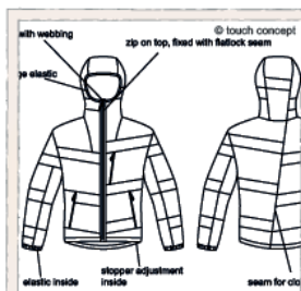
Down jacket -Technical details
